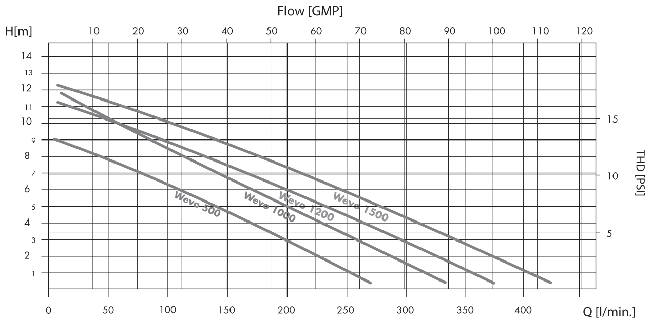
Charakteristika čerpadel WEVO Characteristic of WEVO pumps
